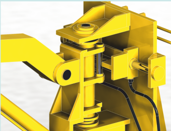
Unique Arm Link Design for Load Distribution
